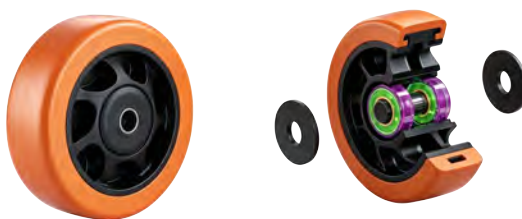
Double Bearing Orange PU Wheel
